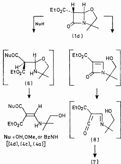
SCHEME Pathways for degradation of the \beta -lactam (1d) [leading to (4a, c, or d) or (7)]
